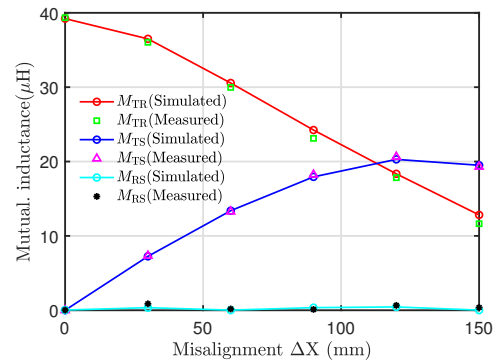
Fig. 16. Measured mutual inductance of proposed RSP coupler versus misalignments along X-axis.
