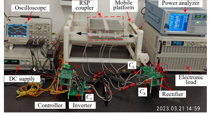
Fig. 15. Experimental prototype of 1-kW IPT system with RSP coupler.
