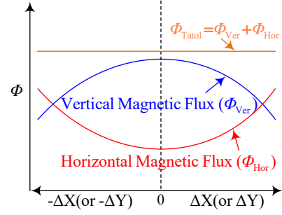
Fig. 1. Complementary design concept.
