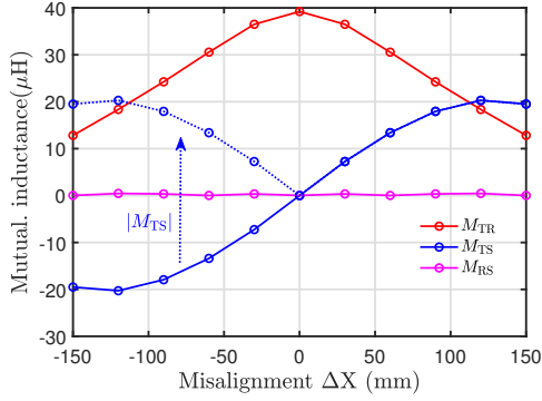
Fig. 13. Mutual inductance polarity of RSP coupler.
