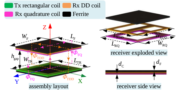
Fig. 5. Commonly-used double-D-quadrature pad (DDQP).
