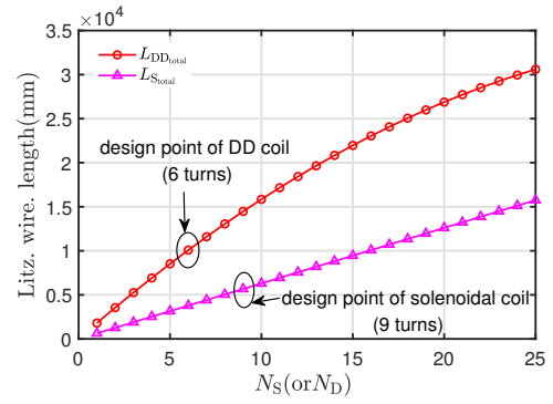
Fig. 11. Total wire length of solenoidal coil and DD coil versus N_S (or N_D ).
