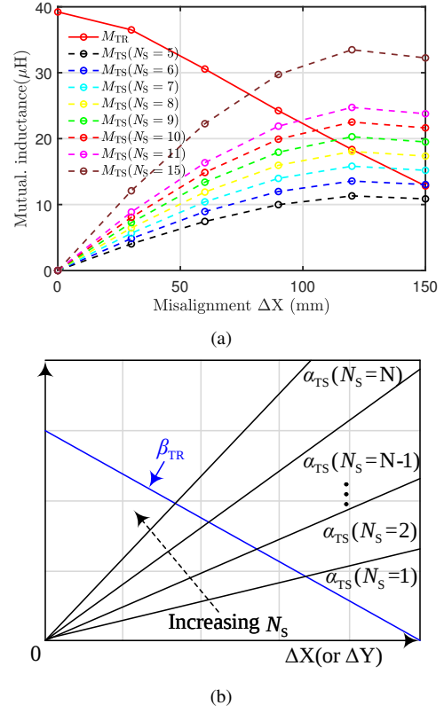
Fig. 8. (a) Mutual inductances M_{TR} , M_{TS} , and (b) approximate slope matching design principles of the proposed coupler with RSP under various misalignments along X-axis versus N_S .
