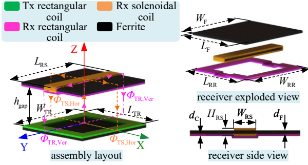
Fig. 2. Proposed rectangular-solenoidal pad (RSP).
