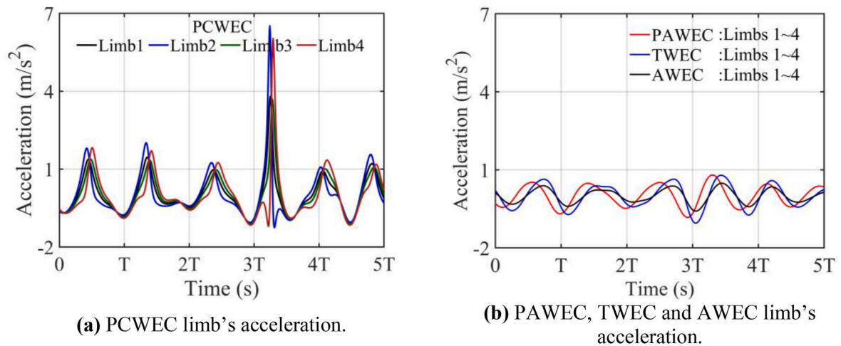
Fig. 15. Power generation limb's acceleration variations for different WECs, in C_{pto} = 40 kN/m, T = 8 s, and H_{1/3} = 2 m.
