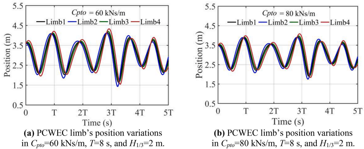
Fig. 19. Power generation limb's position variations for PCWEC under different PTO damping coefficients and certain wave states.
