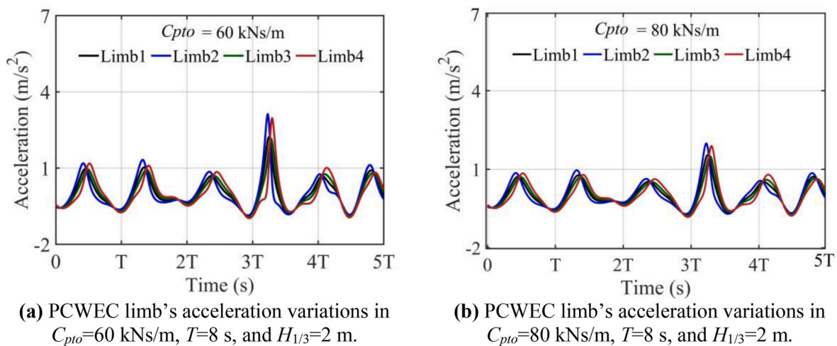
Fig. 21. Power generation limb's acceleration variations for PCWEC under different PTO damping coefficients and certain wave states.
