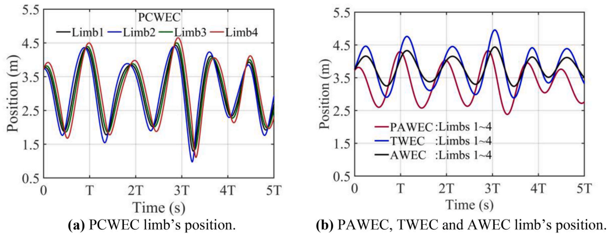
Fig. 13. Power generation limb's position variations for different WECs, in C_{pto} = 40 kN/m, T = 8 s, and H_{1/3} = 2 m.
