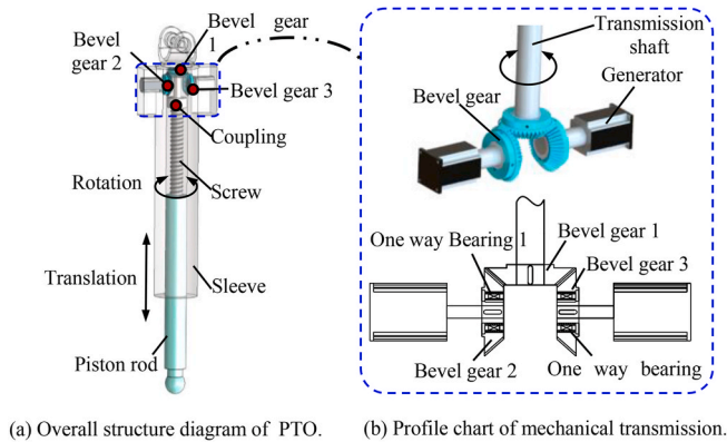
Fig. 4. Mobile self-rectifying PTO design.
