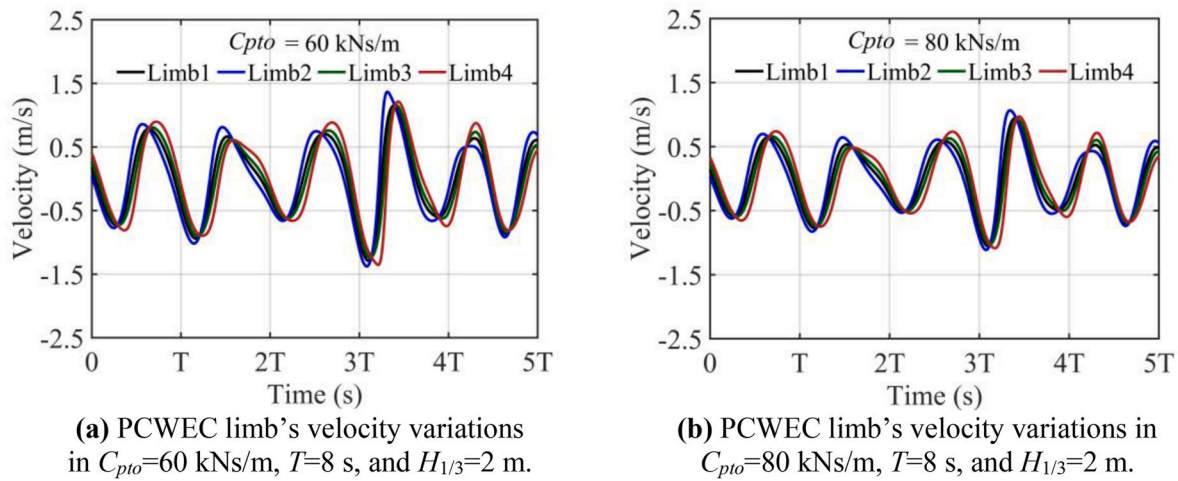
Fig. 20. Power generation limb's velocity variations for PCWEC under different PTO damping coefficients and certain wave states.
