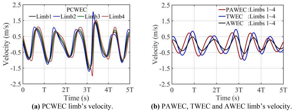
Fig. 14. Power generation limb's position variations for different WECs, in C_{pto} = 40 kN/m, T = 8 s, and H_{1/3} = 2 m.
