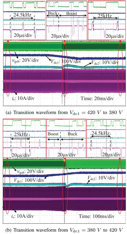
Fig. 15. Transition waveforms between Forward-Buck and Forward-Boost mode of the BSRC with V_{dc2} = 48 V .
