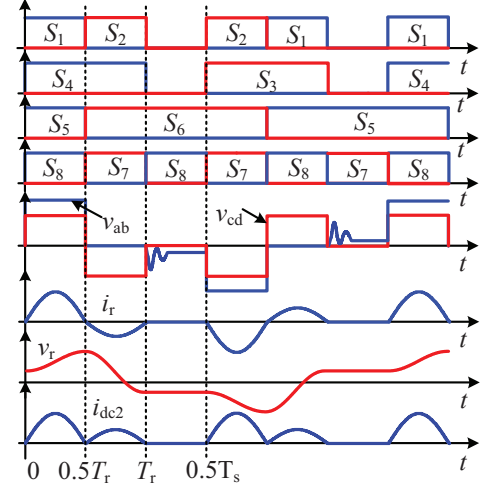
Fig. 3. Switching sequence and operating waveforms of the BSRC in Forward-Buck mode.
