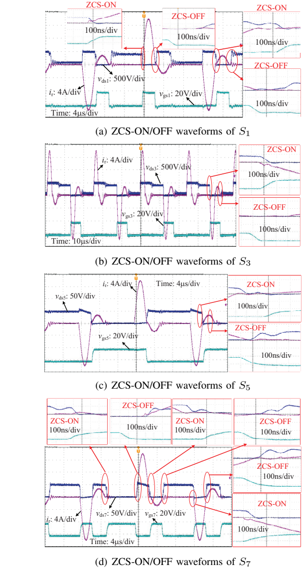
Fig. 11. ZCS-ON/OFF waveforms of the BSRC for Forward-Buck mode.
