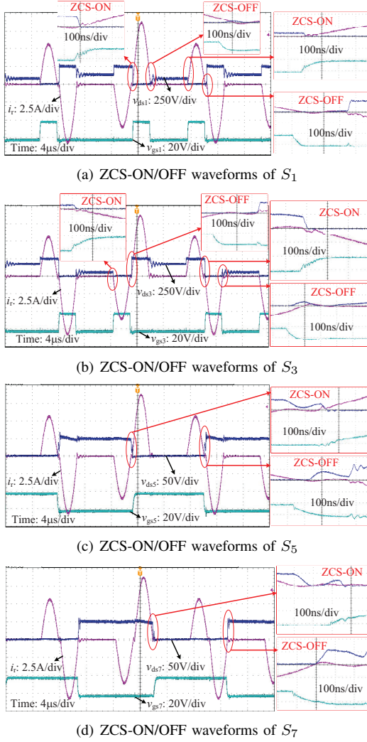
Fig. 13. ZCS-ON/OFF waveforms of the BSRC for Forward-Boost mode.
