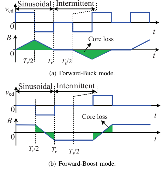
Fig. 8. Waveforms of transformer voltage and magnetic flux density.
