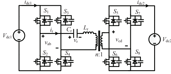
Fig. 2. Schematics of the bidirectional series resonant converter.
