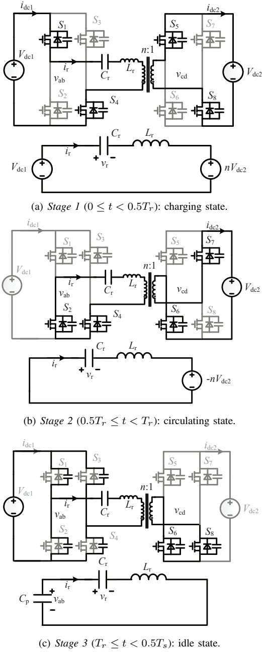
Fig. 4. Equivalent circuits in different stages for Forward-Buck mode.
