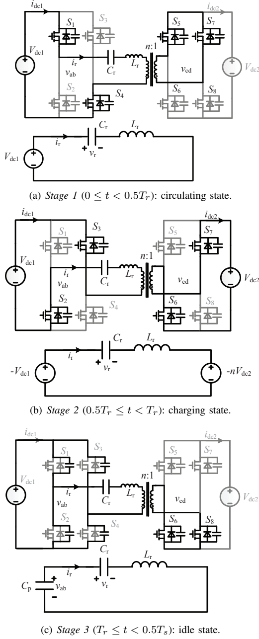
Fig. 6. Equivalent circuits in different stages for Forward-Boost mode.
