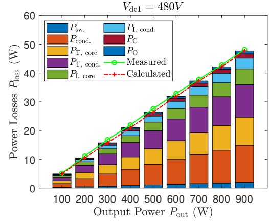
(a) Loss breakdown for V_{dc1} = 480 V and V_{dc2} = 48 V
