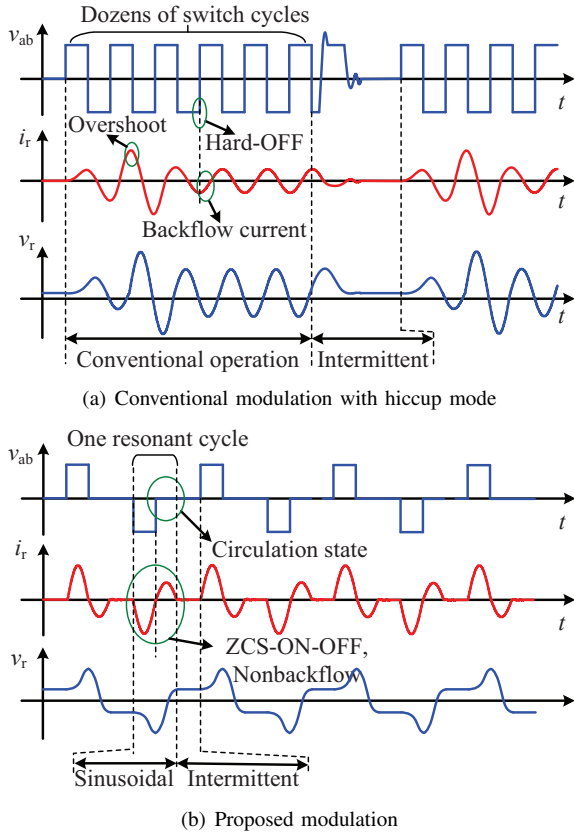
Fig. 1. Basic operating principles of the conventional and the proposed modulations.
