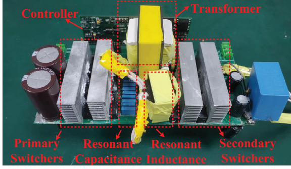
Fig. 9. Photo of the experiment prototype.
