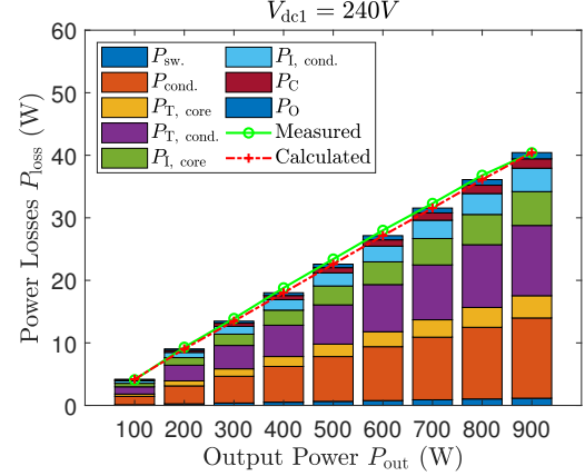
(b) Loss breakdown for V_{dc1} = 240 V and V_{dc2} = 48 V
