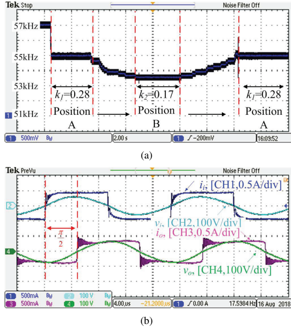
Fig. 12. (a) Reponse of the operating frequency when k dynamically changes from k_1 = 0.28 (position A) to k_2 = 0.17 (position B) and from k_2 = 0.17 (position B) back to k_1 = 0.28 (position A). (b) Experimental waveforms of PP IPT converter.
