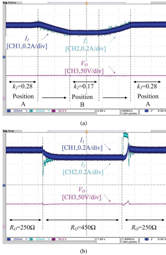
Fig. 13. Transient waveforms of I_1 , I_2 and V_O for (a) k dynamically changing from k_1 = 0.28 (position A) to k_2 = 0.17 (position B) and from k_2 = 0.17 (position B) back to k_1 = 0.28 (position A), at the loading condition R_O = 300 \Omega . (b) R_O step changing from 250 to 450 \Omega and from 450 to 250 \Omega at k = 0.28 .
