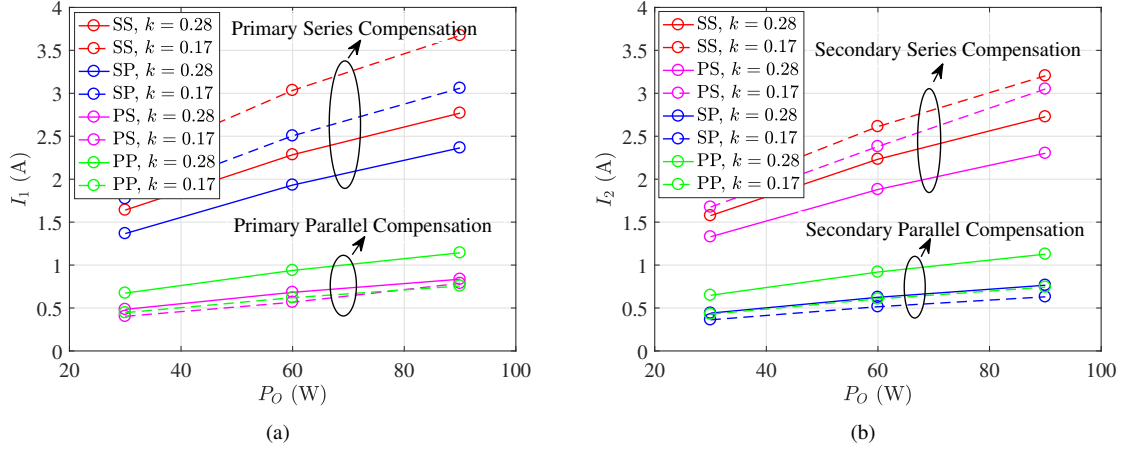
Fig. 10. (a) Measured input current I_1 and (b) measured output current I_2 of the four basic IPT converters at maximum power efficiency points.
