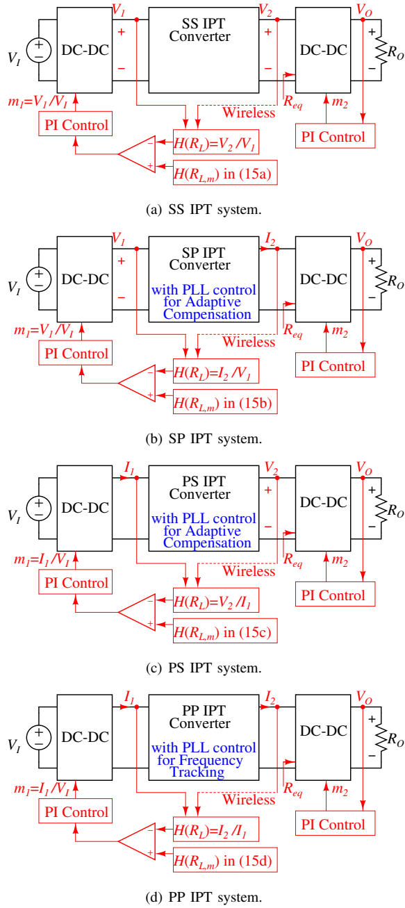
Fig. 5. Control diagrams of the three-stage IPT systems.
