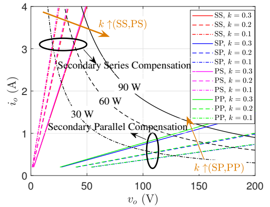
(b) SS and PS IPT converters have a much higher diode rectifier driving current.
