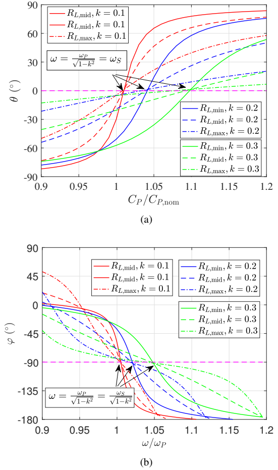
Fig. 4. (a) Input phase angle versus primary compensation capacitance of SP IPT converter. (b) Output phase angle versus operating frequency of PP IPT converter.
